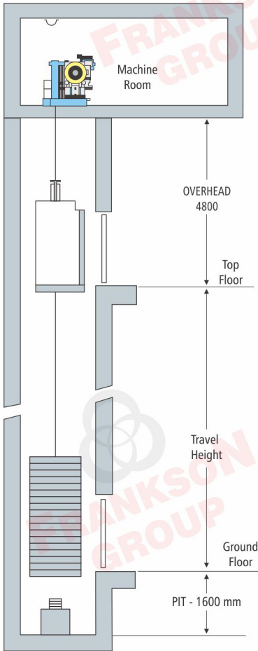
Hoistway Elevation Drawing
